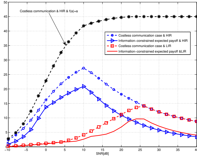
Fig. 4 The difference with Fig. 3 is that the reference power control policy is the semi-coordinated power control policy (SPC), which is already a CPC policy. Additionally, the top curve is obtained with f(a) = a .
