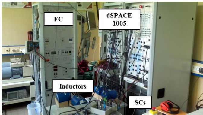
Figure 6: Experimental setup
