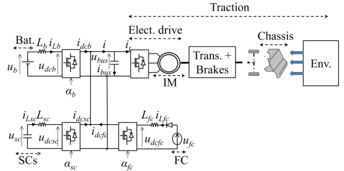
Figure 2: Architecture of the studied vehicle
