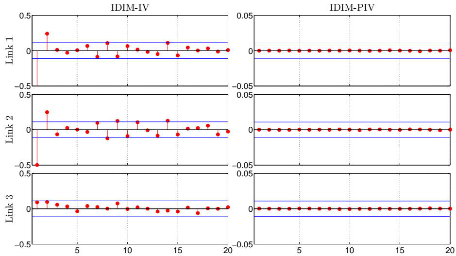
Figure 5: IDIM-IV (left) and IDIM-PIV (right) residuals autocorrelations (red dots) and 2\sigma confidence intervals (blue lines) – Controller known – Axes 1 to 3
