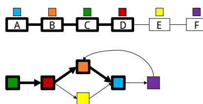
Figure 1. Metabolic clustering. A pattern consisting of four genes (A-D) coding for enzymes that catalyze consecutive reactions (green, red, orange, and blue) is emphasized by thick contours.
