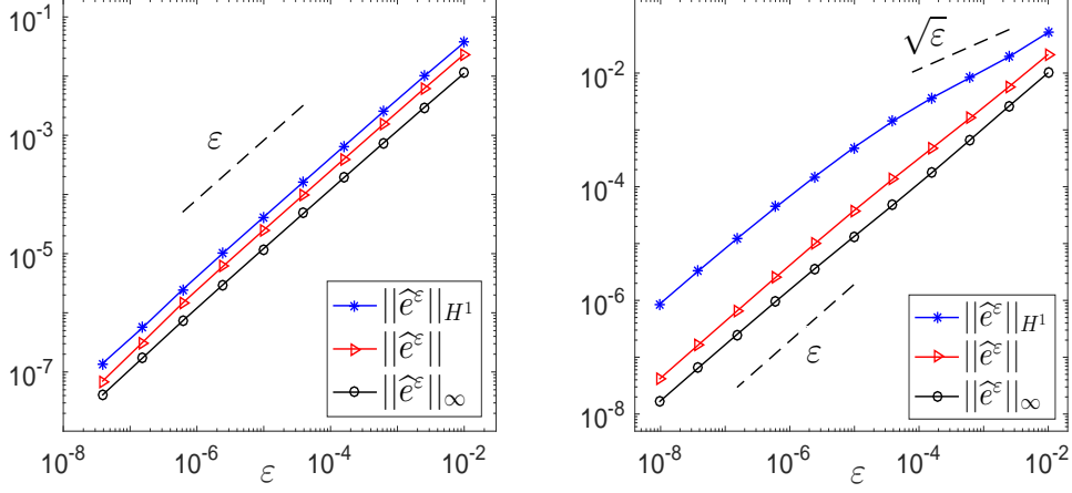
Fig. 4.1: Convergence of the RLogSE (2.1) to the LogSE (1.1), i.e. the error \hat{e}^\varepsilon(0.5) in different norms vs the regularization parameter \varepsilon for Case I (left) and Case II (right).
