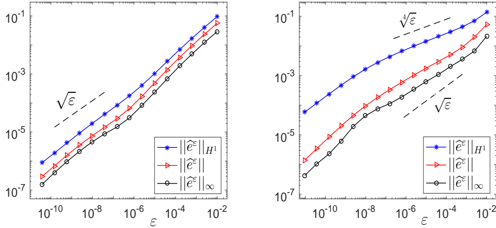
Fig. 4.3: Convergence of the RLogSE (2.8) to the LogSE (1.1), i.e. the error \widehat{e}^\varepsilon(0.5) in different norms vs the regularization parameter \varepsilon for Case I (left) and Case II (right).
