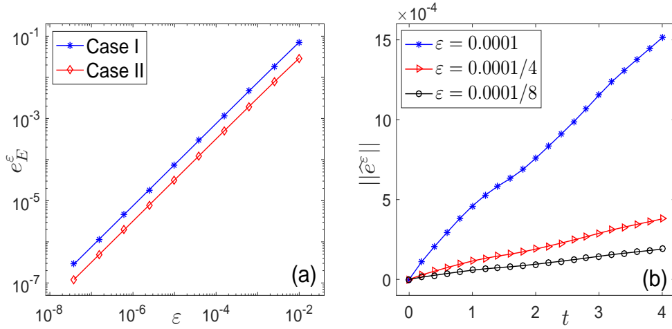
Fig. 4.2: Convergence of the RLogSE (2.1) to the LogSE (1.1): (a) error in energy e_E^\varepsilon(0.5) vs \varepsilon for Cases I & II, and (b) time evolution of \|\hat{e}^\varepsilon(t)\| vs time t under different \varepsilon for Case I.
