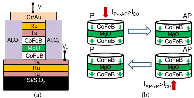
Figure 3. (a) Vertical structure of an MTJ nanopillar composed of CoFeB/MgO/CoFeB thin films. (b) Spin transfer torque switching mechanism: the MTJ state changes from parallel (P) to anti-parallel (AP) as the positive electron flow direction I_{P->AP} > I_{C0} , on the contrast, its state will return as the negative electron flow direction I_{AP->P} > I_{C0} .
