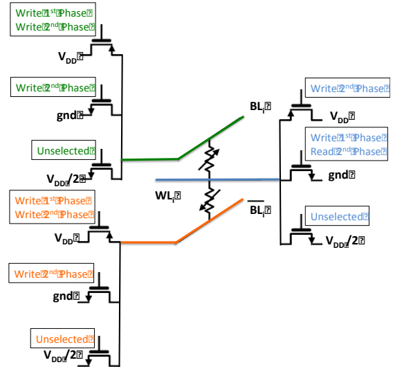
Figure. 8. Bit-line and word-line driver description. Two NMOS and one PMOS are connected to each bit-line and word-line to ensure correct biasing during all phases of operation (Write 1st and 2nd phase, Read 1st and 2nd phase).
