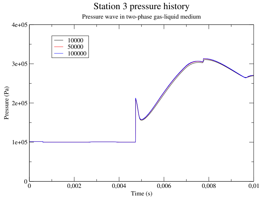
Fig. 13 Two-phase shock tube apparatus with liquid water droplets. Mean pressure signal at station 3. Meshes : 10^4 cells (black), 5 \times 10^4 cells (red) and 10^5 cells (blue)
