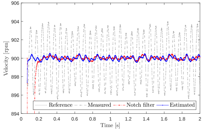
Fig. 7. Measured versus filtered and estimated velocity at 900 rpm using 60 events. Adaptive gain \gamma = 500 .
