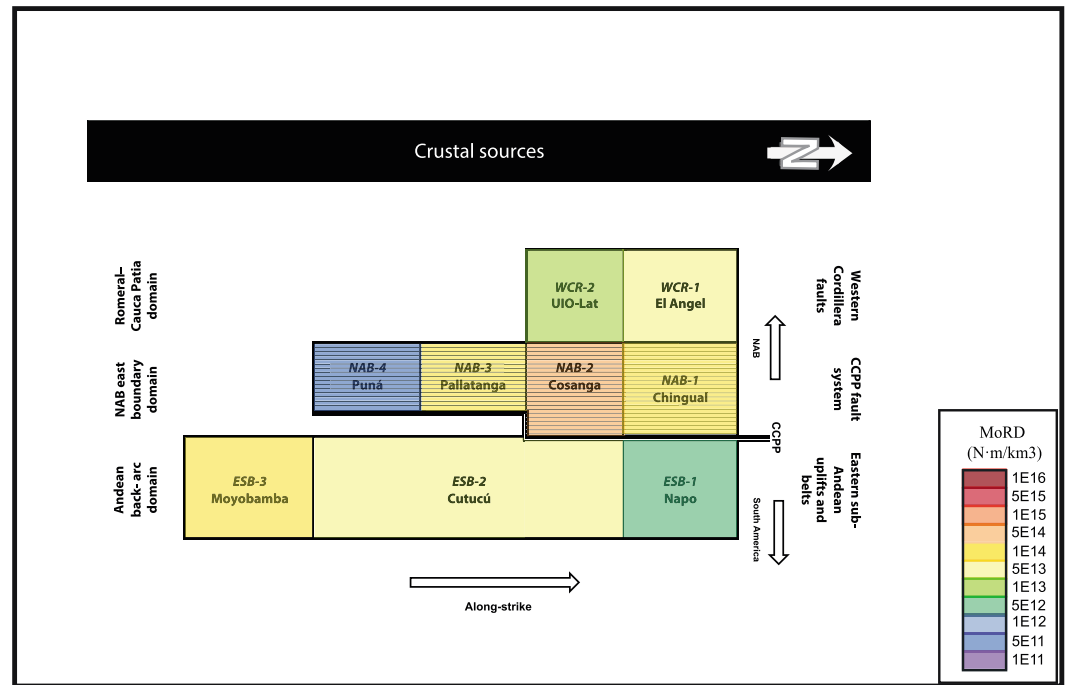
Figure 11. Schematic representation of crustal SSZs. The North Andean Block (NAB) and South American plate boundary is shown as the CCPP fault system. Shaded sources represent the boundary sources. SSZs are colored according to their Mo release density (MoRD).
