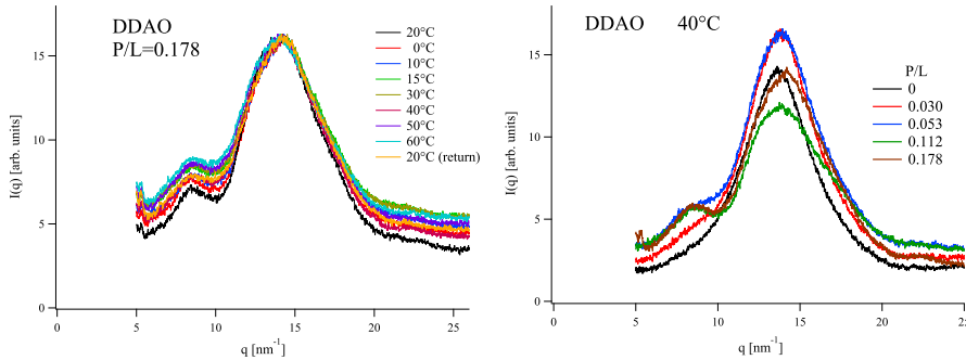
Fig. 6 Scattered signal I(q) for DDAO bilayers, as a function of temperature for the most concentrated sample, with P/L = 0.178 (left) and for all concentrations at T = 40 \text{ °C} (right).
