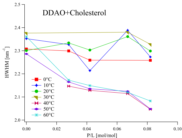
Fig. 10 HWHM as a function of the concentration P/L , for all measured temperatures in the GramA/DDAO+Cholesterol/ H_2O system.
