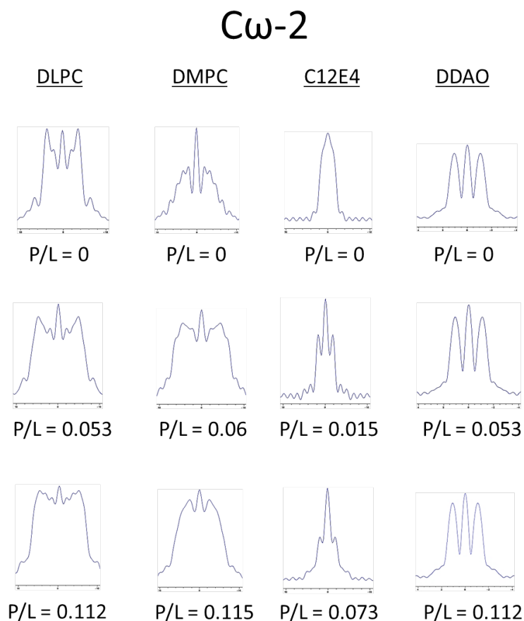
Fig. 2 Dipolar coupling slices of the C_{\omega-2} at 30 °C.
