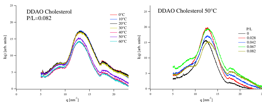
Fig. 8 Scattered signal I(q) for DDAO/Cholesterol bilayers, as a function of temperature for a sample with P/L = 0.082 (left) and as a function of concentration at T = 50^\circ\text{C} (right).
