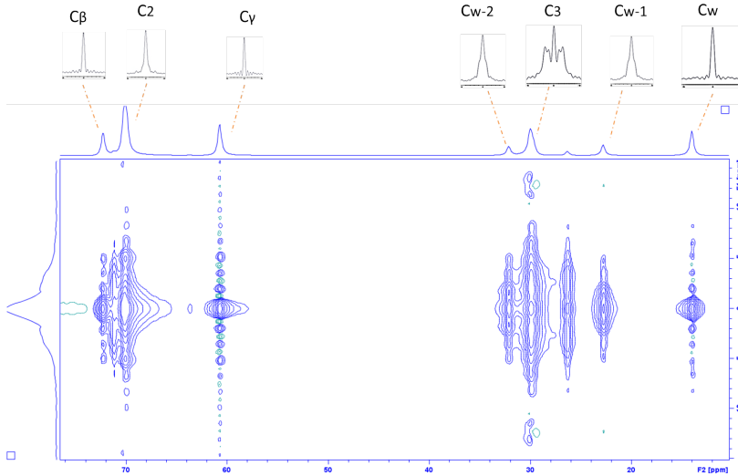
Fig. 1 Example of a 2D ^1\text{H} - ^{13}\text{C} DROSS spectrum for GramA/C 12 EO 4 with P/L = 0.118 .
