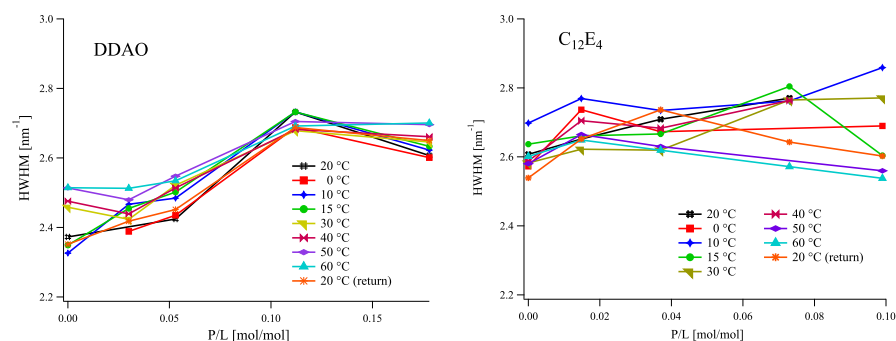
Fig. 9 HWHM as a function of the concentration P/L , for all measured temperatures. DDAO bilayers (left) and C_{12}EO_4 bilayers (right).
