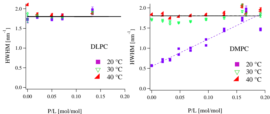
Fig. 5 Width of the chain peak for DLPC (left) and DMPC (right) bilayers as a function of the GramA doping at three temperatures.
