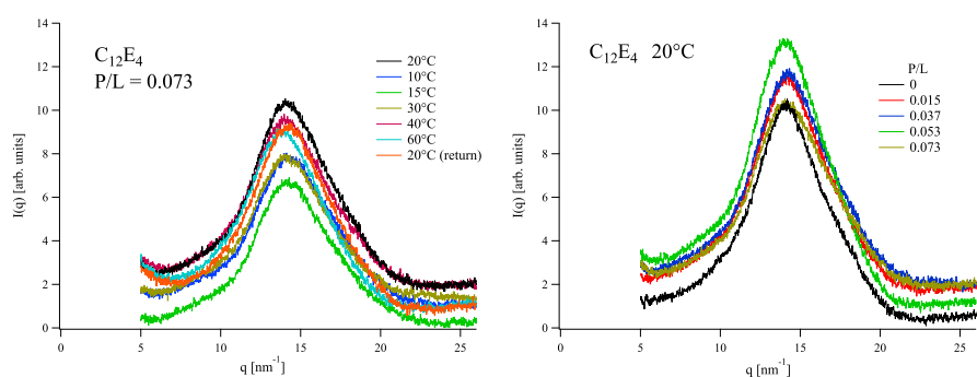
Fig. 7 Scattered signal I(q) for C_{12}EO_4 bilayers, as a function of temperature for a sample with P/L = 0.073 (left) and as a function of concentration at room temperature: T = 20^\circ\text{C} (right).
