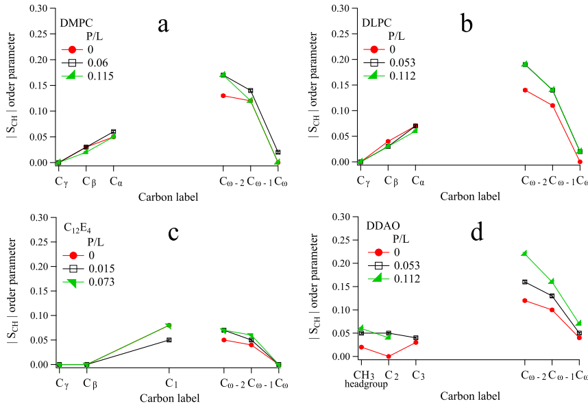
Fig. 3 Orientational order parameter |S_{CH}| for DMPC (a), DLPC (b), C_{12}EO_4 (c) and DDAO (d) bilayers embedded with GramA pores for different P/L at 30^\circ C . Error bars are smaller than symbol size.
