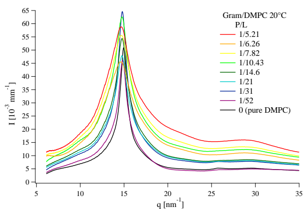
Fig. 4 Chain peak for DMPC in bilayers doped with varying amounts of GramA at 20\text{ }^{\circ}\text{C} .
