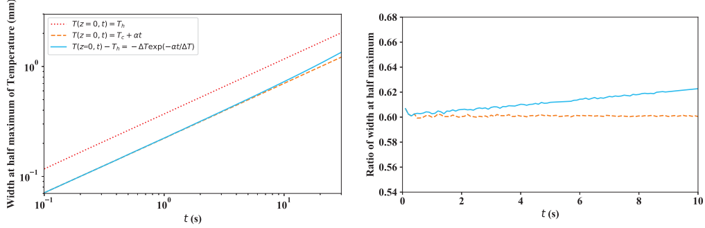
FIGURE 18. Left: numerical width at half maximum of the temperature profiles for three different boundary conditions using a constant temperature at the boundary, Eq. A 9 and Eq. A 10; Right: ratio of the width at half maximum between the rising-temperature cases and the constant-temperature case.
