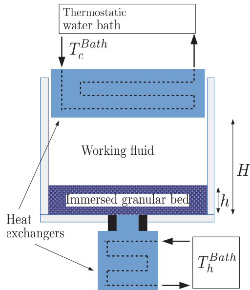
FIGURE 1. Schematic of the experimental setup. The heating coil appears at the bottom while a water circulation allows for refrigeration in the upper side.
