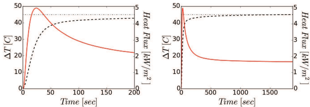
FIGURE 3. Time evolution of measured heat flux density (solid lines) and \Delta T = \Delta T(t, z = 0) (dashed lines) for h = 10 mm; the value of \Delta (see text) is represented by the dot-dashed horizontal lines. Left: early evolution; Right: global time evolution. For the sake of consistency between the different initial layer heights h , the time origin (marked as Time = 0 in the figure) is here chosen as the time (denoted \tau_{ii} , see subsection 3.4) when heat actually reaches the heating metallic plate, i.e. when both \Delta T and the heat flux sharply depart from zero. \Delta being fixed, the maximal slope value for \Delta T (Left Fig.) adopts the same initial value \alpha \simeq 1.25 \text{ K}\cdot\text{s}^{-1} . Temperature and heat flux both settle after a delay of about 700 to 900 s.
