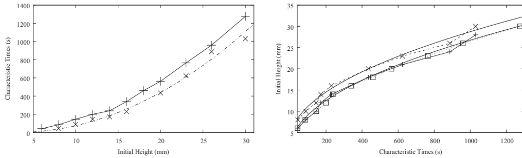
FIGURE 9. Left: Observed characteristic effective heating times for destabilization \tau_h^* ( \times symbols) as compared to destabilization times \tau_h ( + symbols and solid line), both as functions of the initial granular layer thickness h . The \cdots - \cdots line is a least-square quadratic interpolation (1.51 \times (h - 2.96)^2) of the 8 first points of \tau_h^* ( 8 \leq h \leq 23 mm). Right: Initial heights of the granular bed as a function of characteristic times: \tau_h (squares and dotted line), \tau_h^* ( \times and dashed line). The + symbols represents the h values corresponding to \tau_h^* , shifted by 2 mm. The two solid curves are least square quadratic interpolations: respectively h = \nu (\tau + 3) and h = \nu (\tau + 1) , with \nu \simeq 0.814 .
