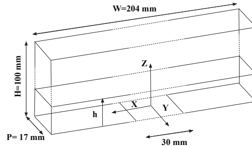
FIGURE 2. Schematic of the inner domain with axis and dimensions. The length of the hot plate is 30 mm.
