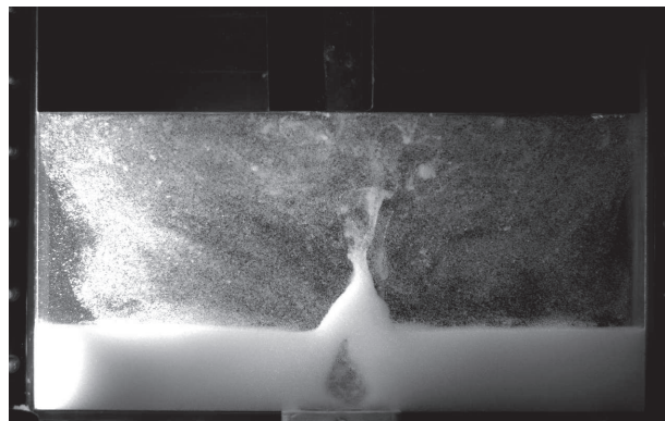
FIGURE 5. Cavity formation at the granular layer, here shown for h = 26 mm and \Delta = 45 K, 450 seconds after the destabilization occurs
