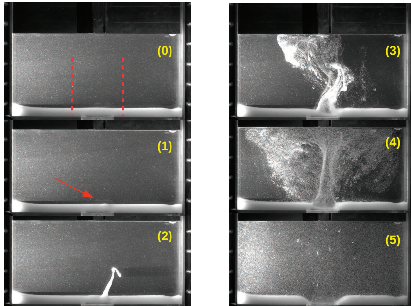
FIGURE 4. Typical destabilization process of the granular layer, here shown for h = 10 mm and \Delta = 45 K. Destabilisation started at t = 147 s. (0) t = 0 : initial situation i.e. up to when heating has just reached the bed's bottom (the two dotted red vertical lines correspond to the analyzed zone for interface evolution monitoring, see text) (1) t = 135 s: precursory deformation of the interface, see the red arrow (2) t = 162 s: granular plume, (3) t = 275 s: plume and beginning of erosion, (4) t = 325 s: erosion and re-deposition of particles, and (5) steady (final) stage with particles' re-deposition left and right from the heating zone and erosion.
