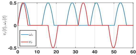
Fig. 1. Reference velocities v_r and \omega_r .
