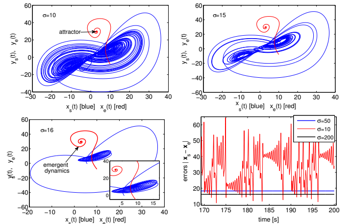
Fig. 5. x - y phase portraits corresponding to the emergent dynamics (28) and the mean-field dynamics (51b) for different values of the interconnection gain \sigma . Bottom-right: |x_s(t) - \bar{x}| .
