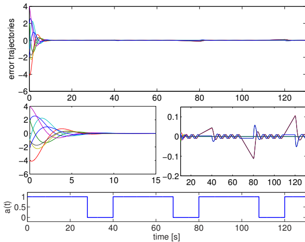
Fig. 1. Mutual synchronization of four Lagrangian systems
