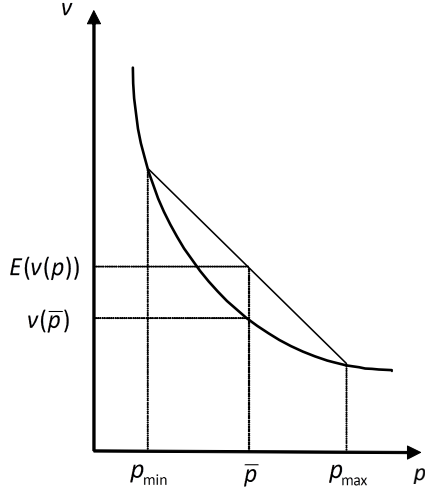
Figure 1a : u_{12} < 0
