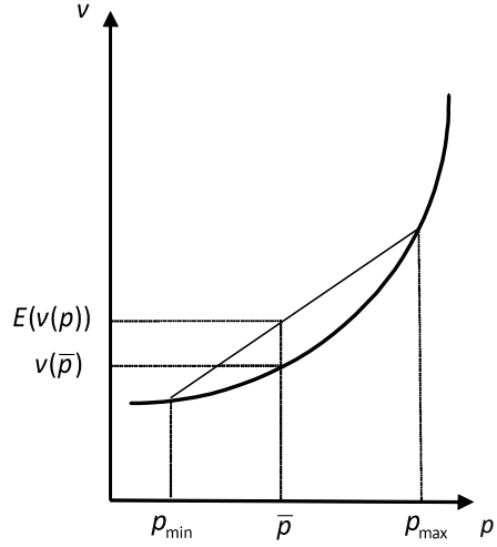
Figure 1b : u_{12} > 0
