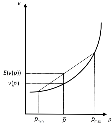
Figure 1b : u_{12} > 0
