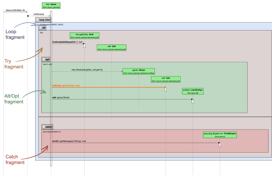
Fig. 6: Sequence Diagram with colored fragments and highlighted message
