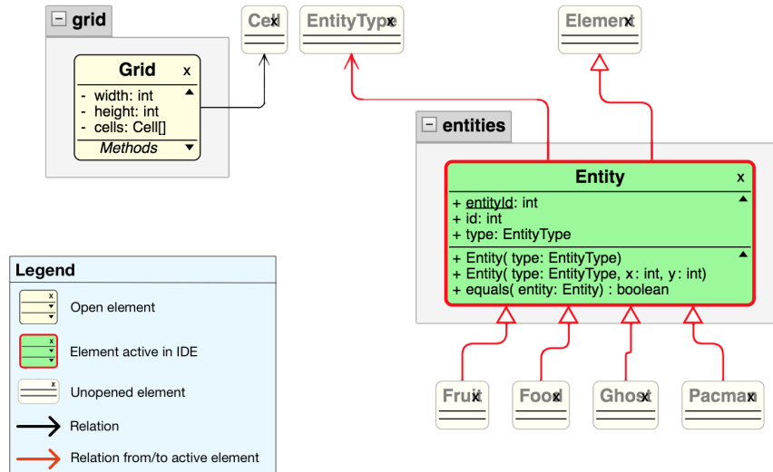
Fig. 4: Class Diagram with unopened related elements and active tab highlighted
