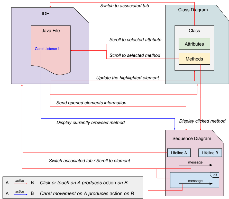
Fig. 3: Navigation interactions and resulting actions
