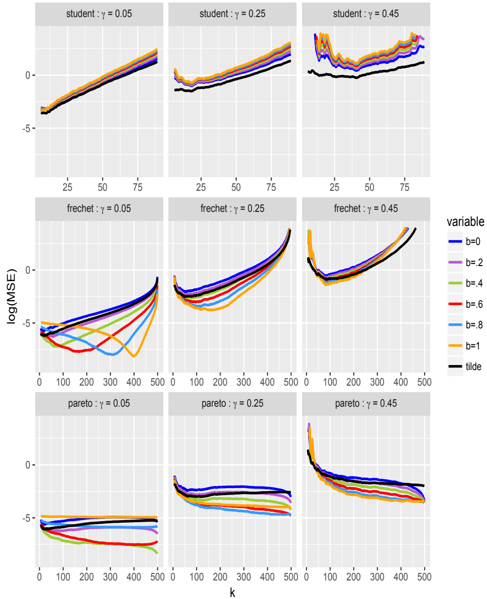
Figure 1. MSE estimates (in log scale) of \widetilde{XES}_{T_n}^*/XES_{T_n} (black) and \overline{XES}_{T_n}^*(\beta)/XES_{T_n} (colour-scheme), against k , for Student (top), Fréchet (middle) and Pareto (bottom) distributions, with \gamma = 0.05 (left), \gamma = 0.25 (middle) and \gamma = 0.45 (right).
