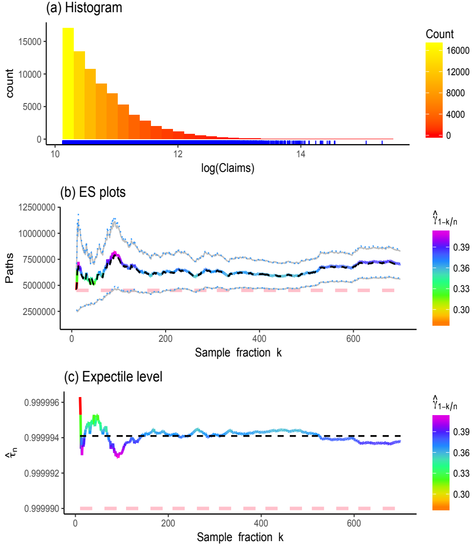
Figure 3. (a) Scatterplot and histogram of the log-claim amounts. (b) The ES plots k \mapsto \overline{XES}_{\hat{\tau}_n^*}(\beta = 1) as rainbow curve, and k \mapsto \widehat{QES}_{p_n}^* in dashed black, along with the constant sample maximum Y_{n,n} in horizontal dashed pink. The confidence intervals \overline{CI}_{0.95}(k) in dotted blue lines and \widehat{CI}_{0.95}(k) in solid grey lines. (c) The plot of k \mapsto \hat{\tau}_n(p_n) as rainbow curve, along with the selected optimal pointwise estimate in horizontal dashed black line, and the constant tail probability p_n in horizontal dashed pink.
