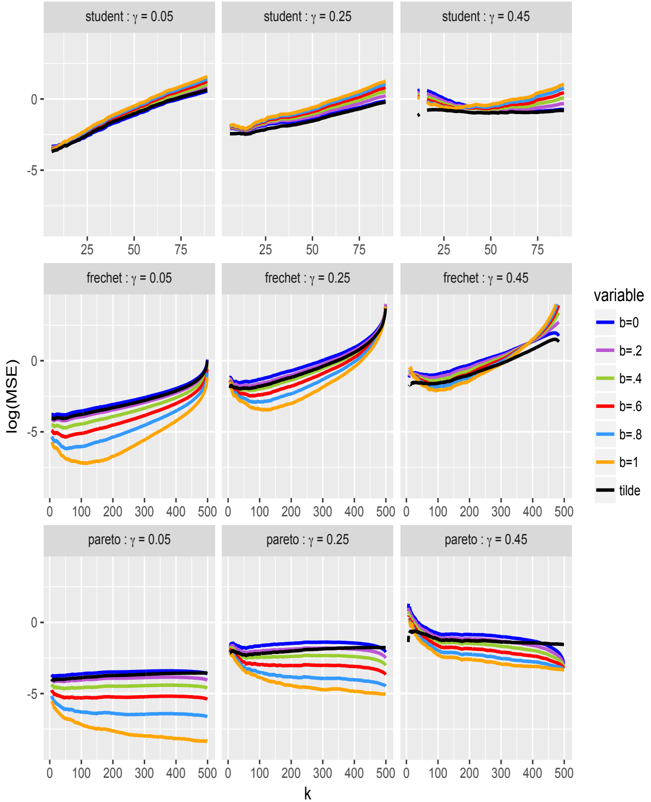
Figure 3: MSE estimates (in log scale) of \widehat{XES}_{\hat{\tau}'_n(p_n)}^*/QES_{p_n} (black) and \widehat{XES}_{\hat{\tau}'_n(p_n)}^*(\beta)/QES_{p_n} (colour-scheme), against k , for Student (top), Fréchet (middle) and Pareto (bottom) distributions, with \gamma = 0.05 (left), \gamma = 0.25 (middle) and \gamma = 0.45 (right).
