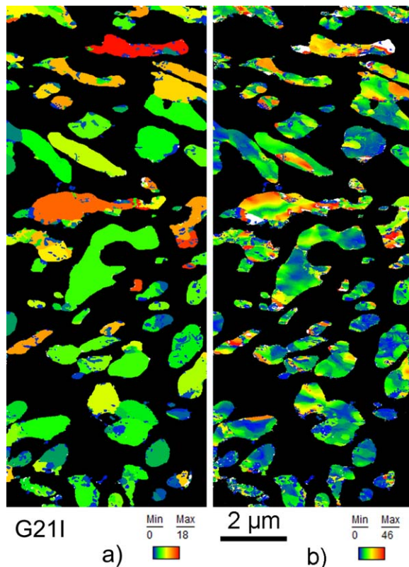
Figure 10. Ferropericlase in G21I (inner position see Figure 1). Total map acquired with a spatial resolution 5 nm-1,200 × 3,000 data points. (a) Grain Orientation Spread (GOS) and (b) Grain Reference Orientation Deviation (GROD) using the average orientation for each grain as the reference (Mis2mean).
