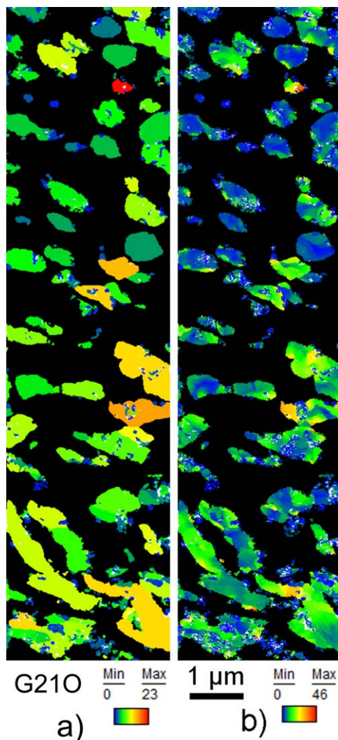
Figure 12. Ferropericlase in G210 (outer position). Total map acquired with a spatial resolution 5 nm-600 × 2,400 data points. (a) Grain Orientation Spread (GOS) and (b) Grain Reference Orientation Deviation (GROD) using the average orientation for each grain as the reference (Mis2mean).
