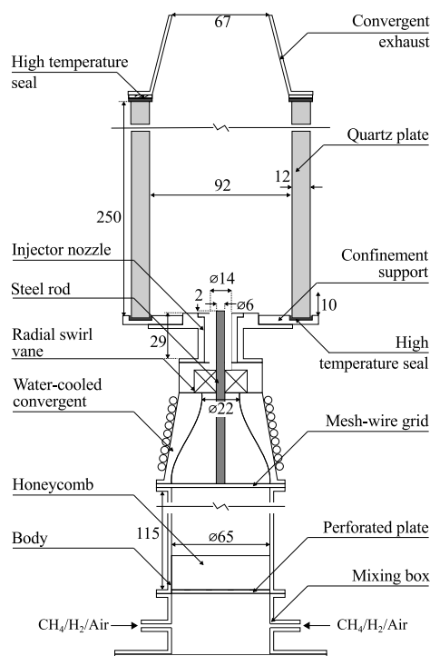
Fig. 6 Schematic view of the studied burner [18,17,33].
