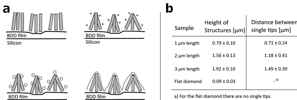
Fig. 1 (a) Sketch of DCNT production: top left: growth of CNTs on BDD film. Top right: hydrophilisation of CNTs. Bottom left: annealing of diamond crystals. Bottom right: growing of diamond layer. (b) Table with information about actual height and pitch of the DCNT structures.
