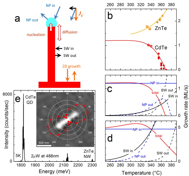
FIG. 4. (a) Scheme of the different contributions to the growth of the NW; the role of the different components of the incident flux (top right) is identified by their color (orange: normal component J_s contributing to the 2D growth and calibrated through RHEED oscillations; black: component J_s \tan \alpha normal to the NW axis impinging the NW sidewalls; blue: total flux of intensity J_s / \cos \alpha ) (b) growth rate of the ZnTe and CdTe segments of sample T (solid symbols) and another sample (open symbols), as a function of temperature. The normal incident flux measured on test (001) 2D layers is the same for both, 0.5 \text{ ML s}^{-1} , with \tan \alpha = 0.21 for CdTe and 0.48 for ZnTe; the same unit is used for the growth rate of CdTe and ZnTe in the NW; (c) the four components entering the CdTe growth rate as calculated for the conditions in (b); (d) the four components for a higher flux ( 2 \text{ ML s}^{-1} ) and an oblique incidence ( \tan \alpha = 1 ); (e) photoluminescence spectrum and (inset) polarization diagram superimposed on the image of the NW.
