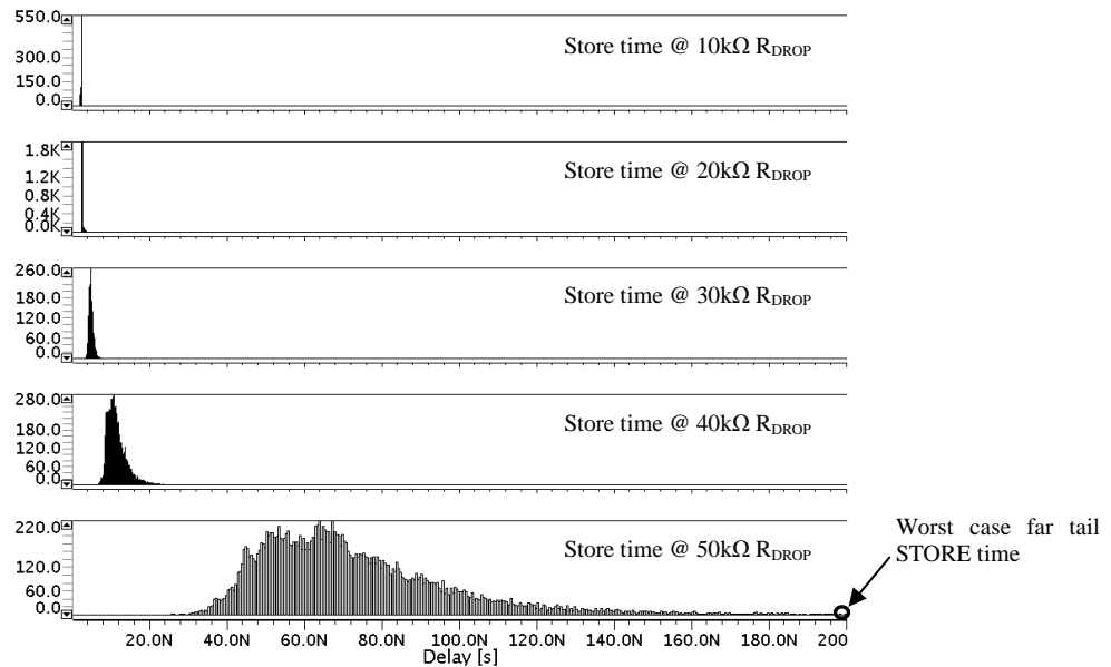
Fig.10 Distributions of STORE time required to obtain various R_{\text{DROP}} in STORE operation obtained from a 10k samples MC simulation for W_{\text{LP}}=100\text{nm} .
