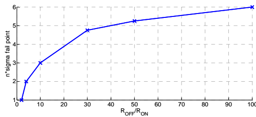
Fig.8 Variation of n*\sigma_{VT} fail point versus the R_{OFF}/R_{ON} ratio in the worst case variation analysis
