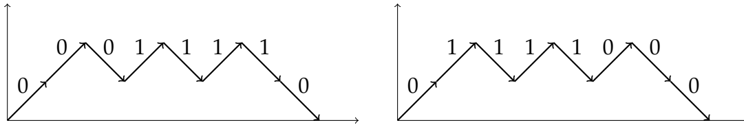
Figure 7: Weighted Dyck paths associated with the prographs of Figure 6 .
