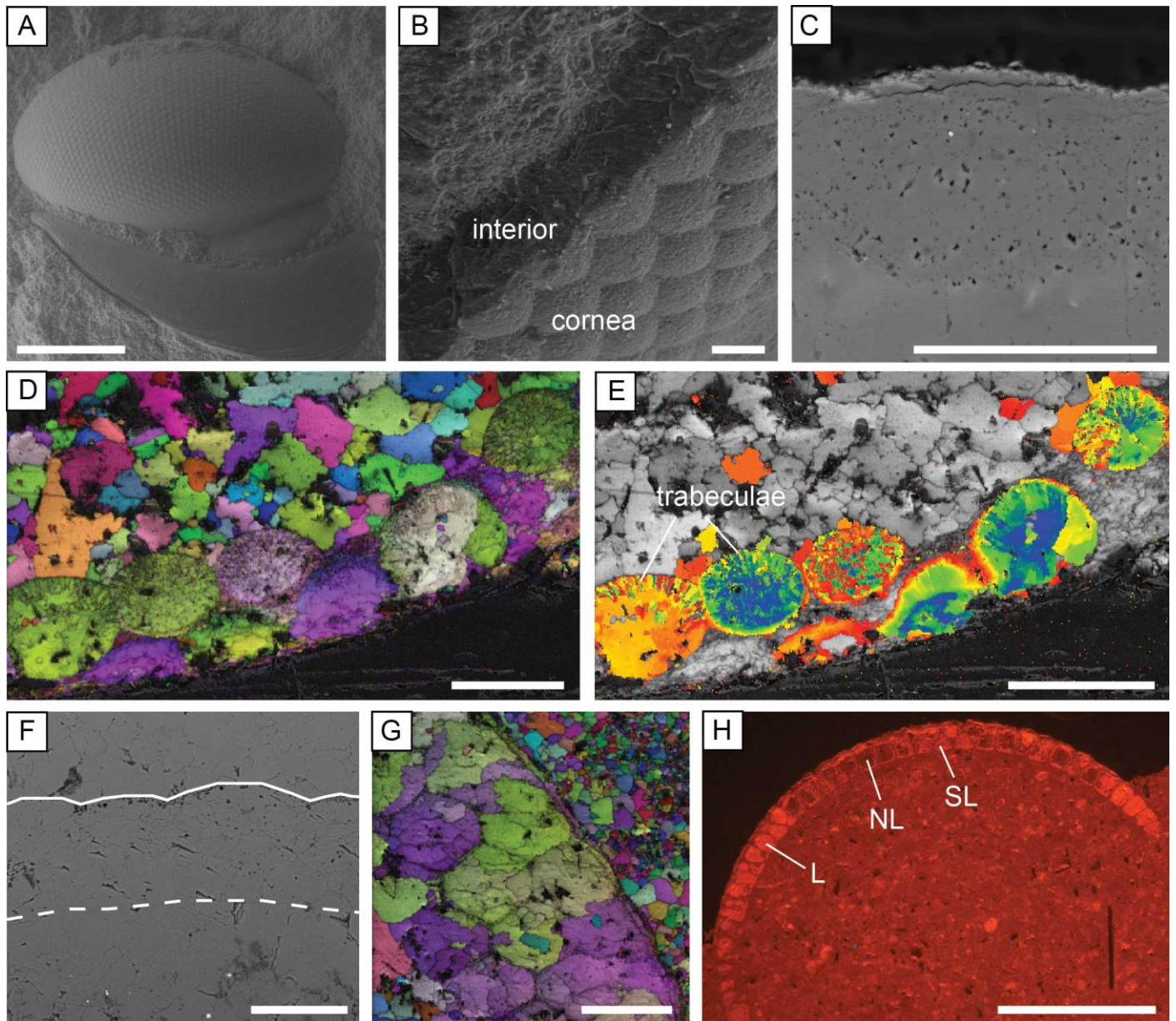
2 Figure 3. Trilobite eye preservation. A: Opipeuterella sp., with intact lenses and libriginal cuticle (specimen 3 T_205_sp4, SE image). B: The recrystallized cornea and interior calcite of the eye lenses (specimen 2.6P, 4 SE image). C: A highly polished telephinid eye lens that contains micro-crystalline dolomite crystals and 5 micro-pitting (specimen T_178_sp10, BSE image). D-E: EBSD images of an asaphid specimen in thin 6 section showing crystallographic continuity within the lenses (D) and the preservation of radial trabeculae 7 structures (E) (specimen A_178_sp1). Image D is an inverse pole figure map overlain on an image quality 8 map, and image E is an orientation tolerance map overlain on an image quality map. F: Lenses that are 9 completely recrystallized, top and base of lenses marked by white lines, the basal boundary is unclear due to
