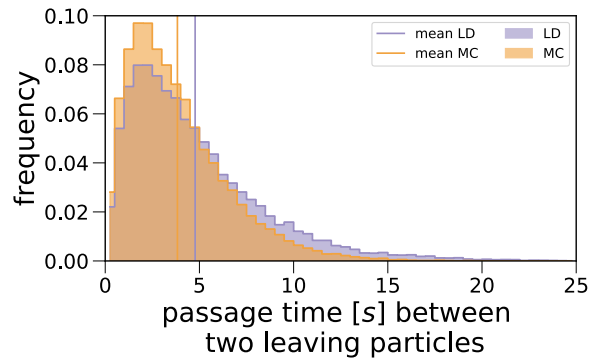
FIG. 6. (Color online) Histograms of passage times (in seconds) between two consecutive particles leaving the lattice (same parameters of Fig. 5). The vertical lines represent the measured 1/J values, giving the timescale of the current.
