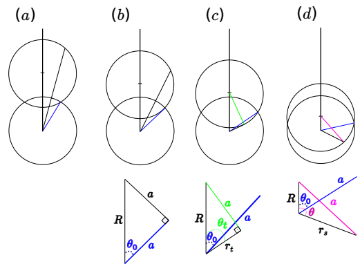
FIG. 8. Sketches of two intersecting spheres with varying distance R between the centres.
