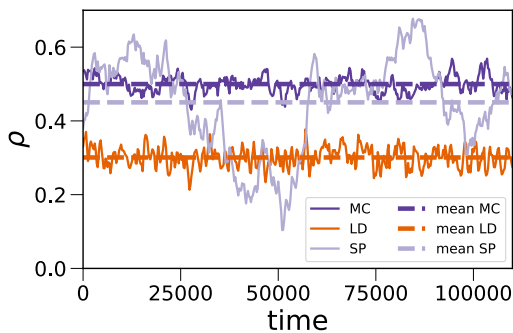
FIG. 7. (Color online) Density of particles as a function of time for LD and MC phases and the SP regime, with \tau = 250 s. For the SP regime \alpha = \beta = 0.1 \text{ s}^{-1} , and the other parameters are the same as the ones used in Fig. 5.
