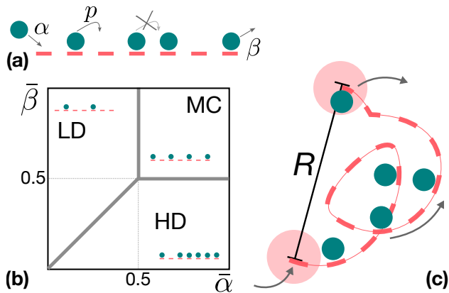
FIG. 1. Scheme of the standard exclusion process (a) and its phase diagram (b), where we emphasised in each phase a typical configuration of the lattice. The same process on a polymer, studied in this paper, is shown in panel (c), where R is the end-to-end distance. Particles are represented by small discs, while large discs represent the reaction volume of the entrance and exit sites (first and last site).
