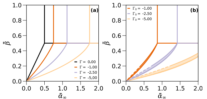
FIG. 2. (Color online) (a) Phase diagram of the TASEP coupled with the diffusive reservoir in the \{\bar{\alpha}_{\infty}, \bar{\beta}\} plane for different values of \Gamma , and (b) phase diagram of the TASEP on a flexible polymer for different values of \Gamma_0 , fixing a = 1.5 , \ell = 1 , l_p = 0.1 and L = 25 (giving R_0 \simeq 2.24 ). All lengths are expressed in lattice-site units. We plug Eqs.(12) in (7) to compute the transition lines; when the lattice is compact d < 1 we use dashed lines and a full line otherwise. The shaded areas in between the LD \rightarrow SP and HD \rightarrow SP transition lines highlight the extended coexistence region.
