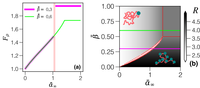
FIG. 4. (Color online) Transport effects on polymer conformation. Panel (a) shows F_\rho = R/R_0 as a function of \bar{\alpha}_\infty , with the shaded region indicating the extended SP. In (b), a color map of the end-to-end distance R (in lattice-site units) in the \{\bar{\alpha}_\infty, \bar{\beta}\} plane. The horizontal lines correspond to \bar{\beta} = 0.3 (magenta, dark gray) and \bar{\beta} = 0.6 (green, light gray), for which F_\rho is shown in panel (a) maintaining the same color code. In both panels \Gamma_0 = -2.5 and the other parameters correspond to the ones used in Fig. 2(b). Red (dark thin) lines correspond to the theoretical phase diagram. In the upper left and bottom right corners of panel (b) we sketch cartoons of the polymer configurations with particles (small discs) on it corresponding to those regions of the diagram: stretched polymers (large R ) are found in the TASEP HD phase, while more compact lattices are expected in the LD (compare phases of the standard TASEP phase diagram shown in Fig. 1).
