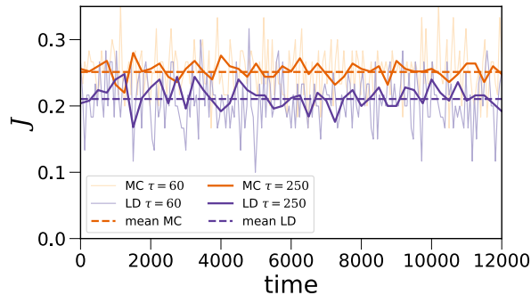
FIG. 5. (Color online) Current J(t) for a TASEP in LD ( \alpha = 0.3 \text{ s}^{-1} , \beta = 0.8 \text{ s}^{-1} ) and in MC ( \alpha = 0.7 \text{ s}^{-1} , \beta = 0.7 \text{ s}^{-1} ). For both cases p = 1 \text{ s}^{-1} and L = 25 (codons). Currents are computed every time interval \tau = 60 s or \tau = 250 s.
