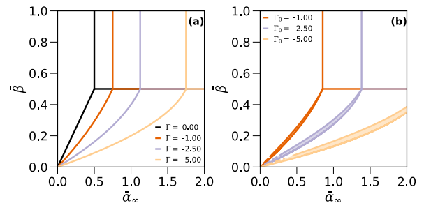
FIG. 9. (Color online) Phase diagrams (equivalent of Fig.2 of the main text) computed with a self-avoiding polymer model R \propto L^{0.588} .
