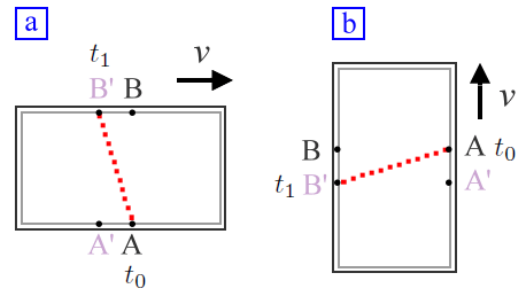
FIG. 5. After rotating 90° (a) Einstein's elevator (b) (let us consider the case in which the elevator travels at constant velocity) we discover what happens to the light beam which is traveling along the vertical arm of the Michelson interferometer, when observed while resting in the ether: the transverse path leans backwards, not in the direction of motion of the system, as usually depicted illustrating the MME. For this reason, in Fig. 1, I specify path in the ref. frame of the ether according to Michelson & Morley [2].
