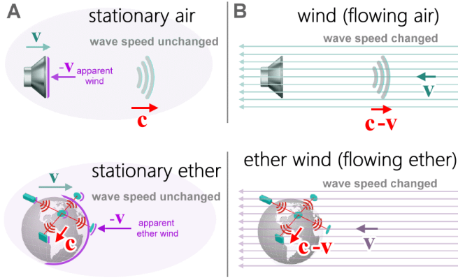
FIG. 3. Difference between wind and apparent wind as regards their action on waves and on massive bodies. In A) only massive bodies traveling through a stationary medium are subject to apparent wind (purple lines indicate the surface of the traveling body which is subject to localized apparent wind), whereas waves (and their velocity, c in the figure) are not affected by apparent wind. Only when the medium is flowing (not stationary), real wind (case B) can change the speed of a wave. Since the MME postulates a stationary ether, apparent wind must be considered instead of real wind, so it emerges that in the MME apparent wind has been erroneously equated to real wind. That's why in the expressions c + v and c - v used to explain the experiment, v has actually to refer only to the speed of the interferometer, not of the ether wind. In this figure c and v refer to velocities not to speeds, so c - v is valid for waves propagating in any direction.
