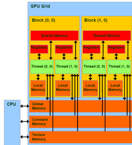
Fig. 1 Cuda architecture
