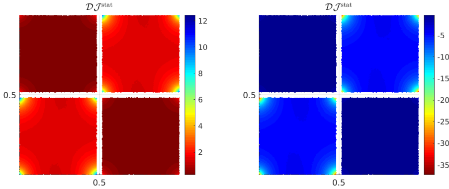
FIG. 4. Distribution of quasi-static sensitivity \mathcal{D}\mathcal{J}^{\text{stat}}(\mathbf{z}) over the unit cell assuming \Delta\mu = 1 (left) and \Delta\mu = -1 (right). The near-interface points are omitted from the plot.
