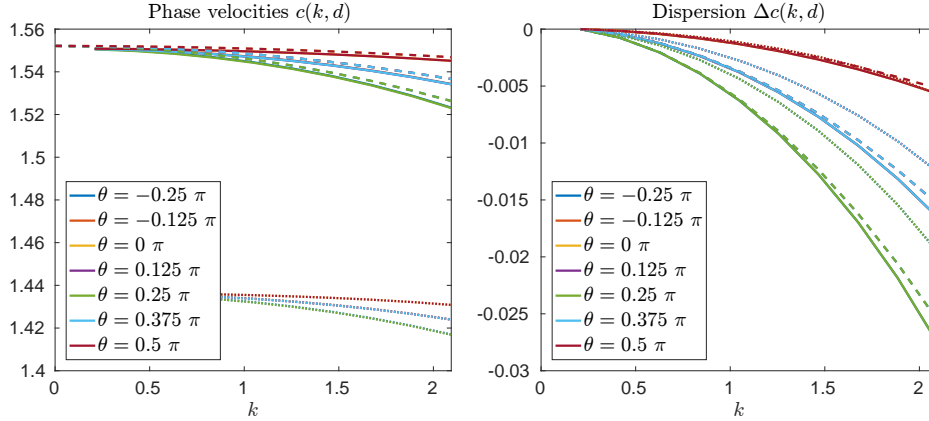
FIG. 3. Left: phase velocity c(k, \mathbf{d}) for the designed chessboard material (homogenized model—dashed, numerical values—solid), and manufactured chessboard material (numerical values—dotted). Right: anisotropic dispersion shown in terms of \Delta c(k, \mathbf{d}) = c(k, \mathbf{d}) - c(k_{\min}, \mathbf{d}) . Note that the results for directions \theta = \{0, \pi/2\} coincide, as do those for directions \theta = \{-\pi/4, \pi/4\} and \theta = \{-\pi/8, \pi/8, 3\pi/8\} .
