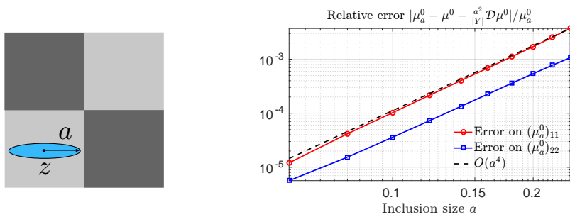
FIG. 1. Approximation of \mu_a^0 by its leading-order topological expansion for a chessboard unit cell perturbed by an ellipsoidal inclusion with \Delta\mu = 1 and semi-axes (a, 0.2a) , centered at \mathbf{z} = (0.25, 0.25) . Left: perturbed unit cell where the light (resp., dark) gray indicates \mu = 1 (resp., \mu = 2 ). Right: relative error made by the leading-order approximation of a \mu_a^0 in terms of its diagonal entries. The mass density of all constituents inside the perturbed unit cell is \rho = 1 .
