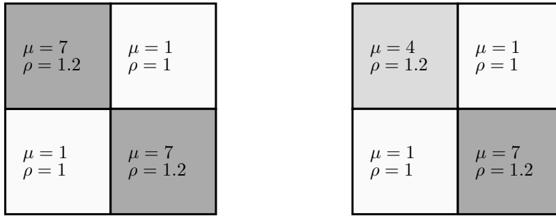
FIG. 2. Designed (left) and manufactured (right) 1 \times 1 unit cell of a chessboard-like material.
