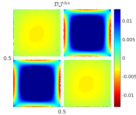
FIG. 5. Distribution of dynamic sensitivity \mathcal{D}\mathcal{J}^{\text{dyn}}(\mathbf{z}) over the unit cell assuming \Delta\mu = -1 . The near-interface points are omitted from the plot, and a threshold is applied to the most positive TS values (as only their sign is of interest) so that the color scale is symmetric around 0.
