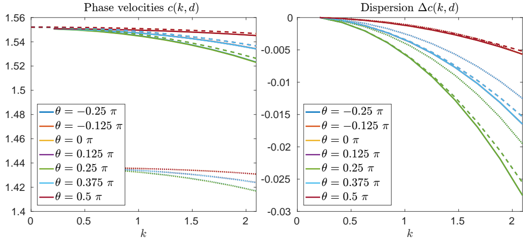
FIGURE 3. Left: phase velocity c(k, \mathbf{d}) for the designed chessboard material (homogenized model - dashed, numerical values - solid), and manufactured chessboard material (numerical values - dotted). Right: anisotropic dispersion shown in terms of \Delta c(k, \mathbf{d}) = c(k, \mathbf{d}) - c(k_{\min}, \mathbf{d}) . Note that the results for directions \theta = \{0, \pi/2\} coincide, as do those for directions \theta = \{-\pi/4, \pi/4\} and \theta = \{-\pi/8, \pi/8, 3\pi/8\} .
