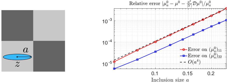
FIGURE 1. Approximation of \mu_a^0 by its leading-order topological expansion for a “chessboard” unit cell perturbed by an ellipsoidal inclusion with \Delta\mu = 1 and semi-axes (a, 0.2a) , centered at \mathbf{z} = (0.25, 0.25) . Left: perturbed unit cell where the light (resp. dark) grey indicates \mu = 1 (resp. \mu = 2 ). Right: relative error made by the leading-order approximation of \mu_a^0 in terms of its diagonal entries. The mass density of all constituents inside the perturbed unit cell is \rho = 1 .
