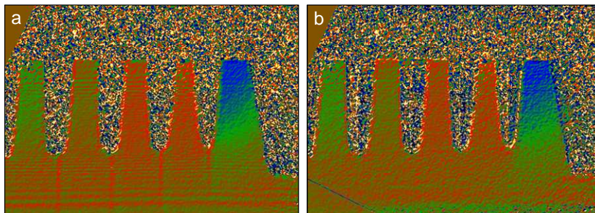
Figure 5. Rotation maps before (a) and after (b) removal of the thickness variation artefacts. The Fresnel fringe artefacts have also been removed from (b) by Fourier filtering.
