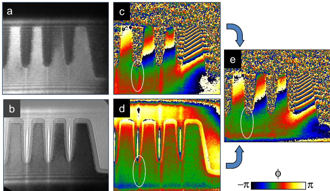
Figure 4. Correction of thickness artefacts: (a) dark-field electron hologram; (b) bright-field hologram; (c) dark-field phase; (d) bright-field phase; (e) subtraction of the dark-field and bright-field phases. Ovals indicate principle artefacts. Fresnel fringes have been removed by Fourier filtering.
