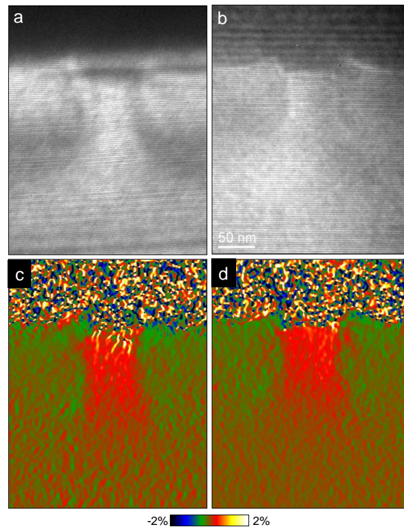
Figure 6. Comparison of pseudo-Lorentz mode (a,c) and aberration-corrected Lorentz mode (b,d). Dark-field electron holograms from the (004) beam (a,b) and corresponding deformation maps (c,d).
