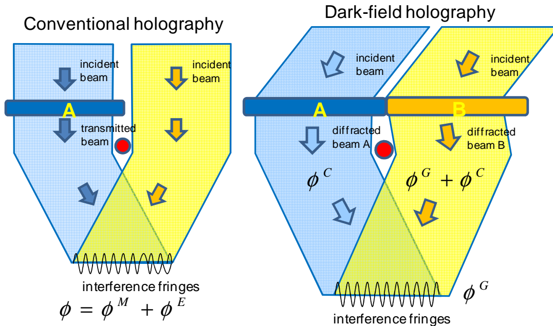
Figure 1. Schematic representation of conventional off-axis holography (left) and dark-field electron holography (right). Transmitted beam in the vacuum, and diffracted beam from unstrained crystal, serve as references for the former and latter respectively.
