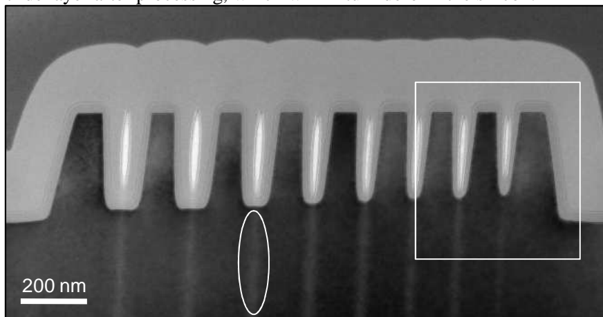
Figure 2. Conventional bright-field image of comb-like Si test structure for \text{Si}_3\text{N}_4 stress liners. Analysed zone (square) and curtaining effect from FIB specimen preparation (oval) indicated.
