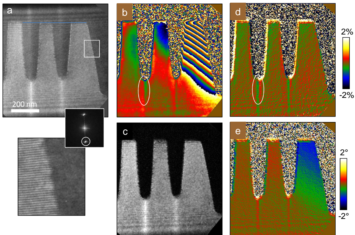
Figure 3. Analysis of dark-field hologram: (a) dark-field hologram from (111) diffracted beam, Fourier transform and zoom inset; (b) phase; (c) amplitude; (d) local variation in planar spacing; (e) local lattice plane rotation.
