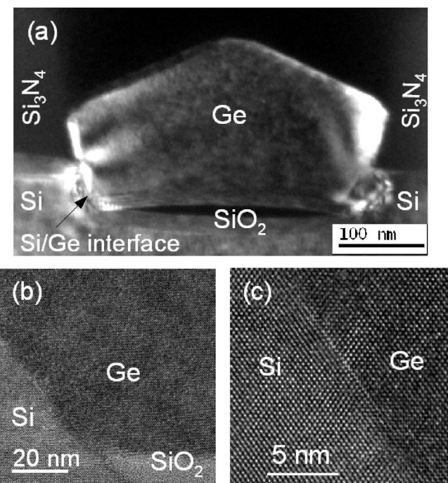
FIG. 3. TEM WBDF images obtained in a g=220 , ( g, -2g ) condition from a Ge crystal (a) and HREM images [(b) and (c)] of the Ge/Si interface.
