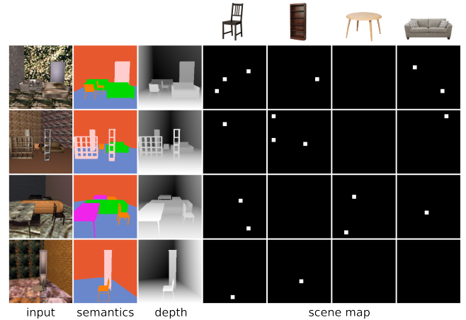
Figure 6: An illustration of 4 samples from the data generation pipeline. We render RGB, semantic segmentation, depth, and scene map, resulting in an unlimited stream of fully defined training data.
