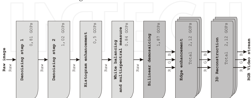
Fig. 2.3. Example a of a low level image reconstruction video pipe.
