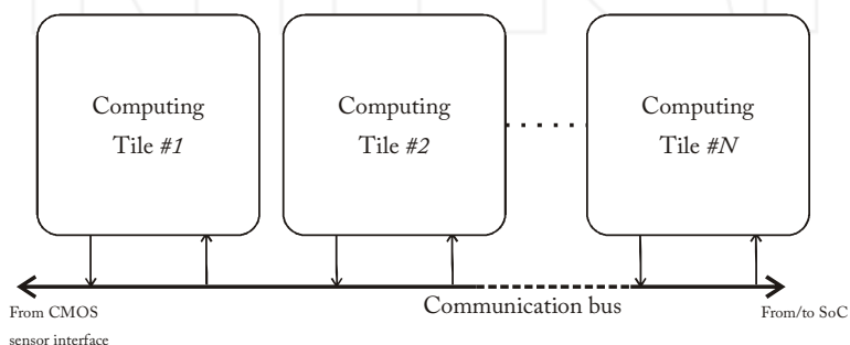
Fig. 3.1. eISP, a computile tile architecture.
