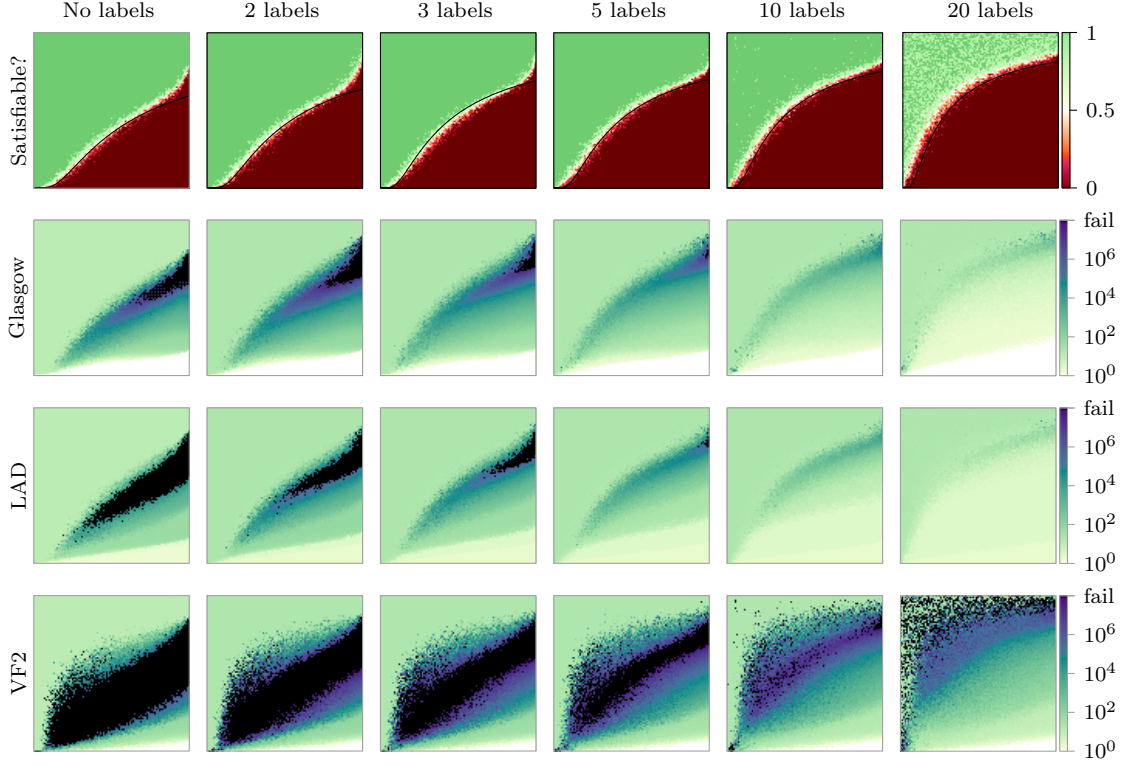
Figure 8: On the top row, predicted and actual location of the phase transition for labelled non-induced random subgraph isomorphism, with a pattern order of 20, a target order of 150, varying pattern (x-axis) and target (y-axis) density, and varying numbers of labels. On subsequent rows, the average number of search nodes needed to solve an instance, for three different solvers
