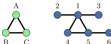
Figure 2: An example used to illustrate the simple constraint programming model for the problem: the pattern graph is on the left, and the target graph on the right.
