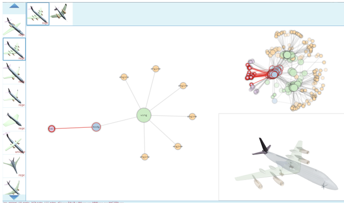
Fig. 6: User Interface. In the left sidebar we show a set of 3D models represented by pre-computed 3D renderings. In the top bar, we show pre-computed 3D renderings of all models that have the same topology as the currently selected one. The main view shows the graph of the selected model while the lower right shows an interactive 3D rendering. The upper right shows an overlay of topologically similar models. The selected node (pink in the main view) is propagated both to the overlay view as well as the interactive 3D view (the tail is highlighted).
