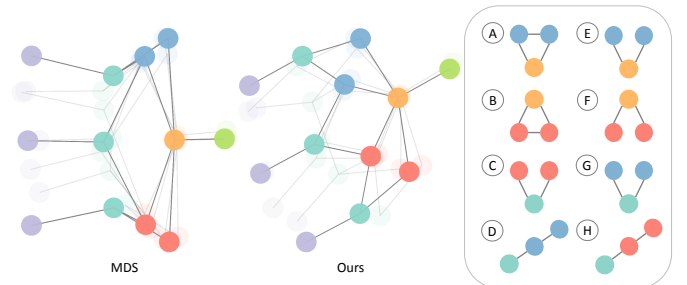
Fig. 8: Sample Task Q7. The user is given a collection of graphs in an overlaid fashion where the graphs are drawn jointly using either the MDS-based method or our method (randomly chosen). Then the user is asked to select from (A-H) the subgraphs that appear in the dominant structure of the given collection. The purpose is to measure how well the user understands the graph collection with the given embedding, which can be further used as a measure of the usefulness of the embedding. In this example, the correct answers are (C,E,F,G). Fig. 9 shows that using our method, 80% of the users can give the correct answer while only 43% of the users give the correct answer using the MDS-based method.
