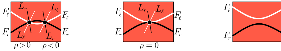
Fig. 5. A transition with “creation/annihilation” of two hyperbonodes.
