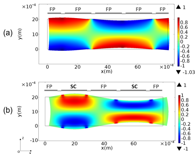
FIG. 5. Calculated color map of the electric potential and mode deformation shape associated to S_0 wave for an infinite Pz26 plate in the xz -plane for: (a) Frequency f=420 kHz and electric boundary configuration 1 and (b) frequency f=388 kHz and electric boundary configuration 2.
