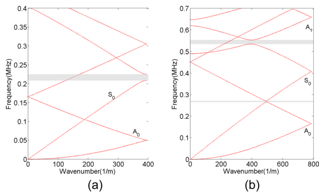
FIG. 6. Calculated band structure for (a) the symmetric EBC configuration whose elementary cell of length \Lambda=8 mm (two FP succeeded by two SC electrodes) and (b) an antisymmetric EBC (configuration 3). The gray-shaded rectangles represent the band gaps regions.
