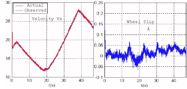
Fig. 9. Estimated velocity using the ABS sensors
