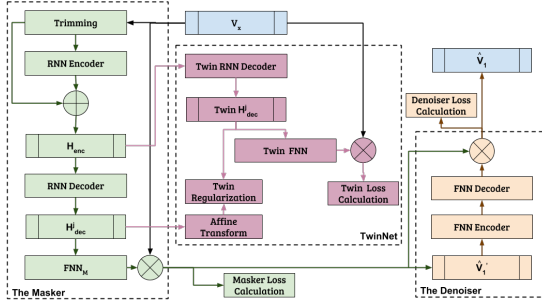
Figure 2: Illustration of the Mad TwinNet system (adapted from [18]). With green color is the Masker, with magenta the TwinNet, and with light brown the Denoiser.
