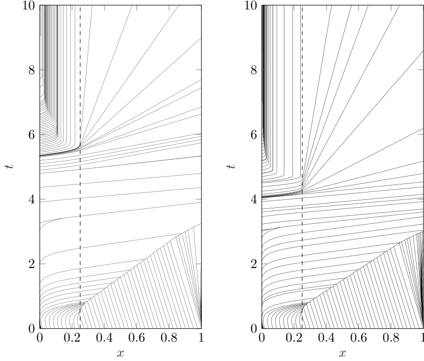
FIGURE 5.2. Evolution of the characteristic curves for Buckley-Leverett flux f_{1/4}^{BL} with \alpha = 0.75 (left) and \alpha = 1 (right)
