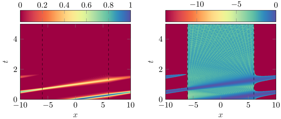
FIGURE 5.7. Evolution of the solution to (5.11) in standard scale (left) and in log scale (right)
