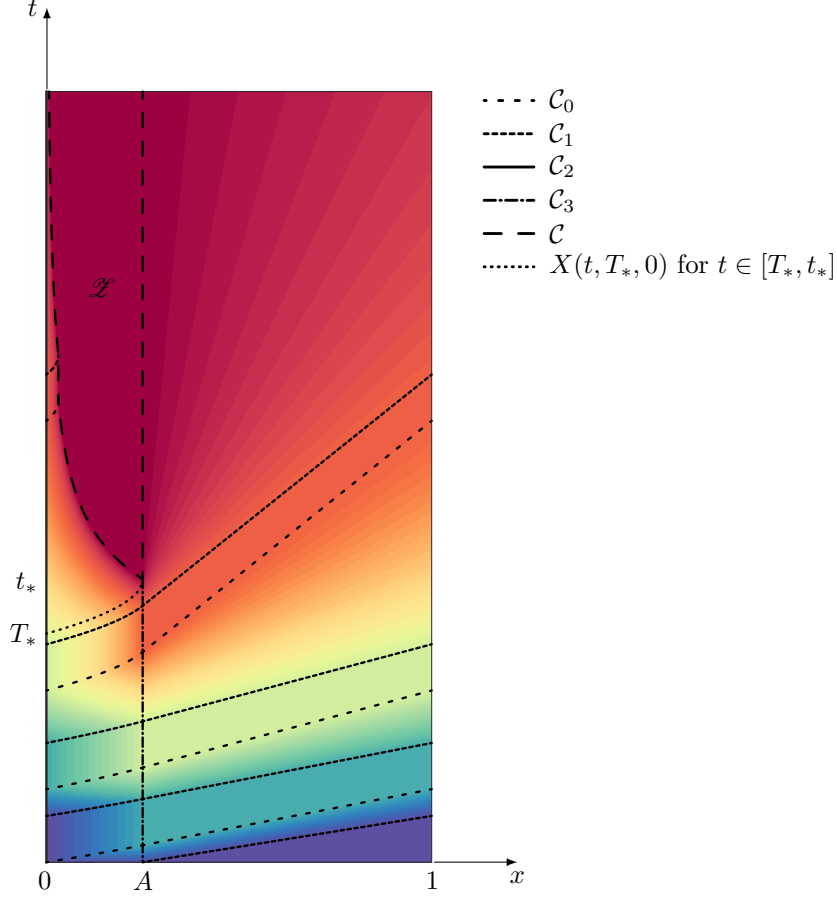
FIGURE 4.2. Discontinuity curves, \mathcal{Z} region and times T_* and t_* .
