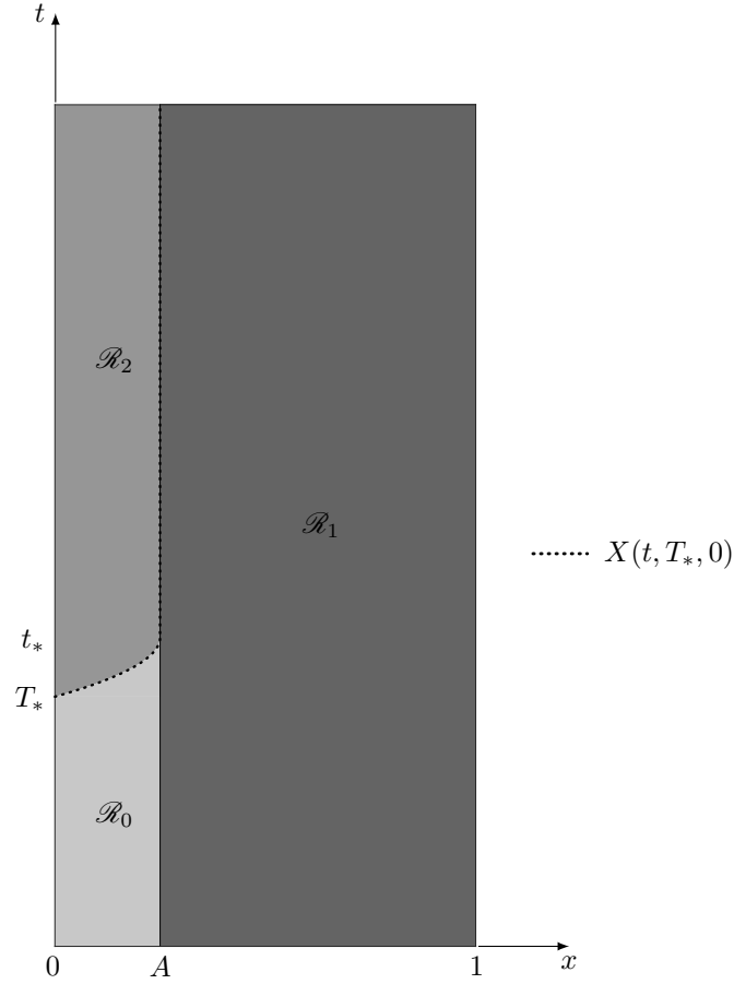
FIGURE 4.3. \mathcal{R}_0 , \mathcal{R}_1 and \mathcal{R}_2 regions.
