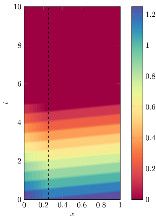
FIGURE 1.1. Evolution of the solution for transport equation
