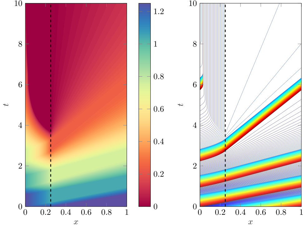
FIGURE 4.1. Evolution of the solution (left) and of the characteristic curves (right) for Burgers flux
