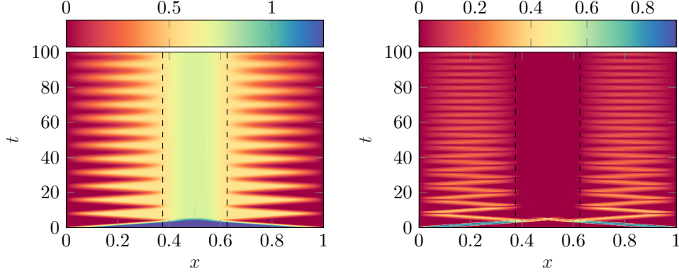
FIGURE 5.5. Evolution of the solution to (5.9), u on the left and \partial_t u on the right
