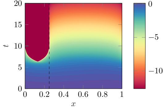
FIGURE 5.3. Evolution of the \log_{10} of the solution to (5.7) with \alpha = 0.75
