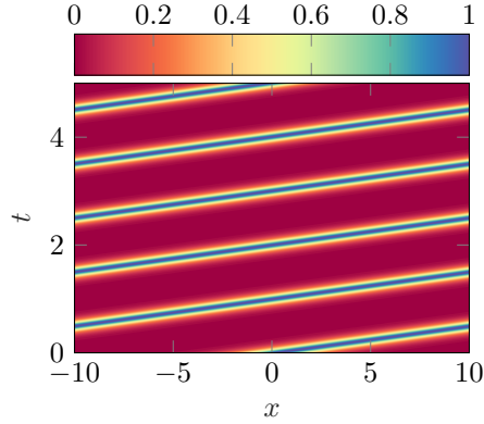
FIGURE 5.6. Evolution of the modulus of the soliton (5.12) for c = 20 and k = 0.81 .
