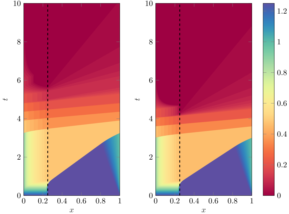
FIGURE 5.1. Evolution of the solution for Buckley-Leverett flux f_{1/4}^{BL} with \alpha = 0.75 (left) and \alpha = 1 (right)
