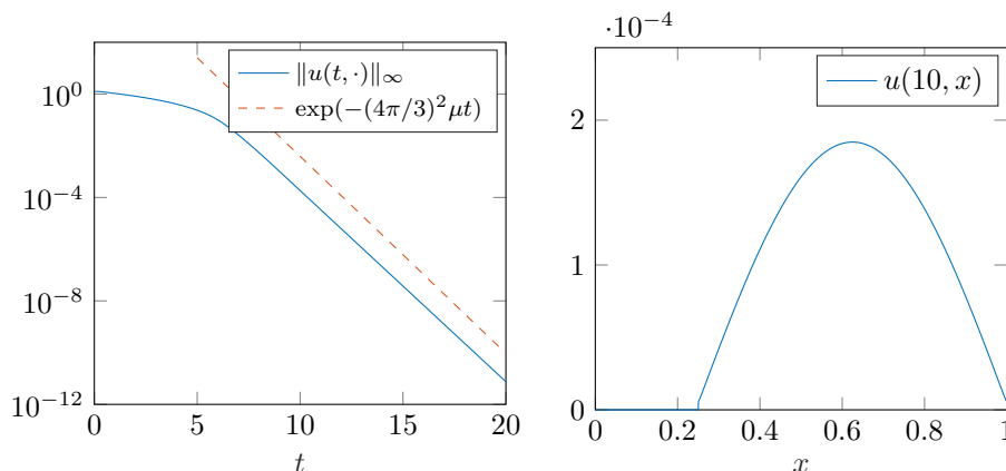
FIGURE 5.4. Evolution of the L^\infty norm of the solution to (5.7) in log-scale (left) and solution at time t = 10 (right) for \alpha = 0.75
