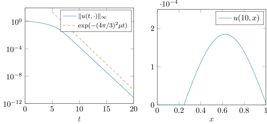
FIGURE 6.4. Evolution of the L^\infty norm of the solution to (6.7) in log-scale (left) and solution at time t = 10 (right) for \alpha = 0.75
