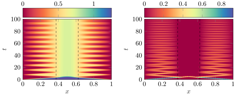
FIGURE 6.5. Evolution of the solution to (6.9), u on the left and \partial_t u on the right
