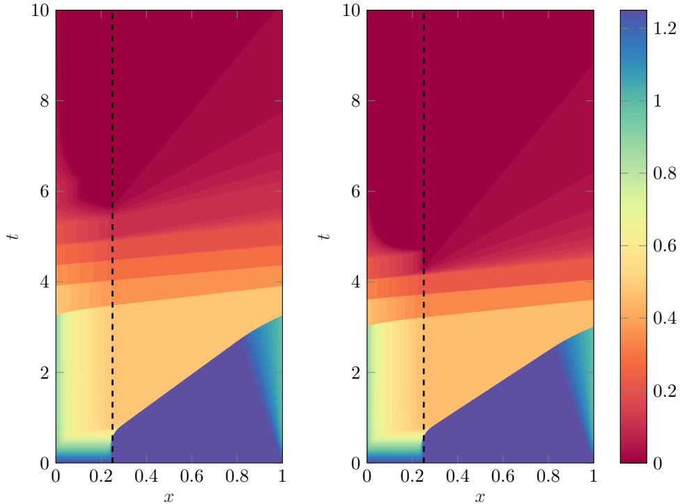
FIGURE 6.1. Evolution of the solution for Buckley-Leverett flux f_{1/4}^{BL} with \alpha = 0.75 (left) and \alpha = 1 (right)
