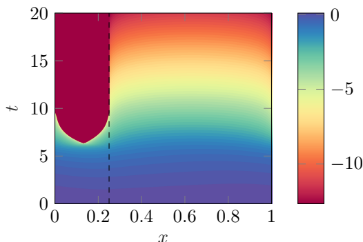
FIGURE 6.3. Evolution of the \log_{10} of the solution to (6.7) with \alpha = 0.75
