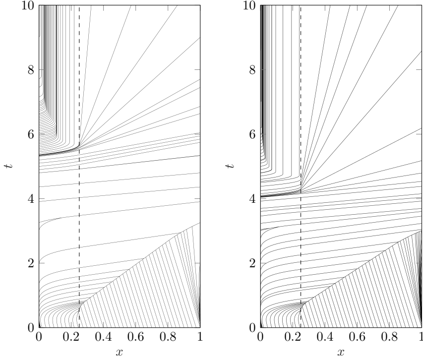
FIGURE 6.2. Evolution of the characteristic curves for Buckley-Leverett flux f_{1/4}^{BL} with \alpha = 0.75 (left) and \alpha = 1 (right)
