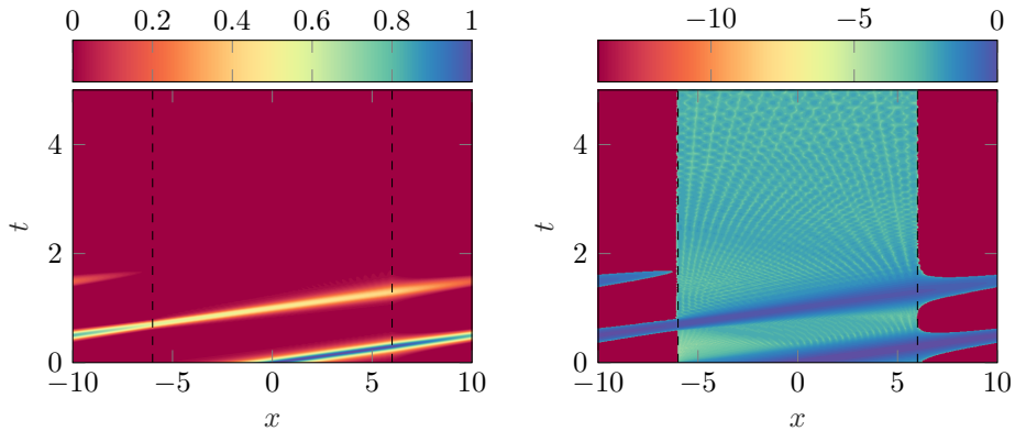
FIGURE 6.7. Evolution of the solution to (6.11) in standard scale (left) and in log scale (right)
