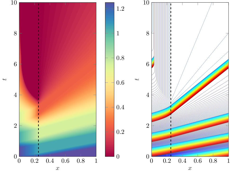
FIGURE 5.1. Evolution of the solution (left) and of the characteristic curves (right) for Burgers flux
