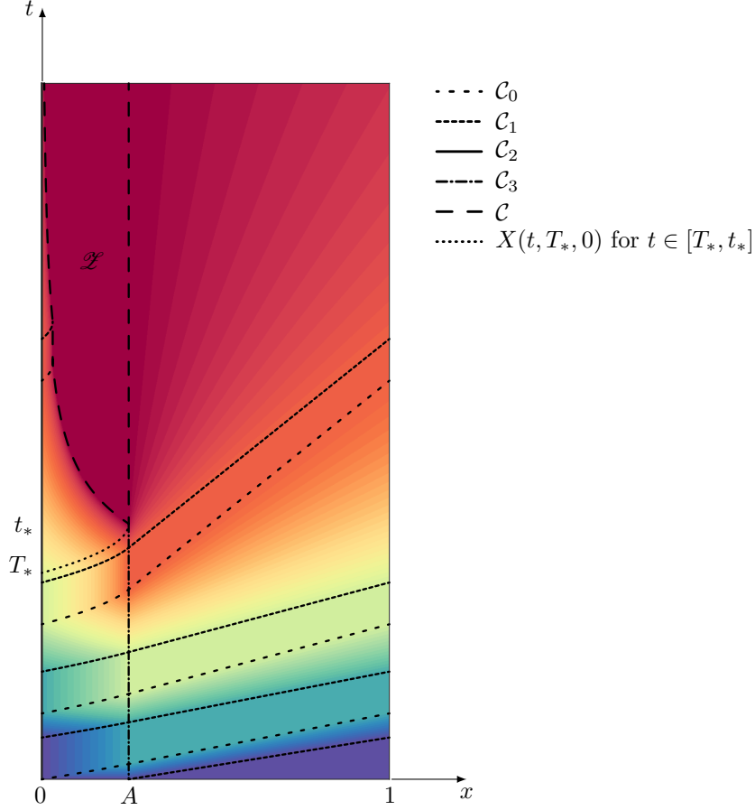
FIGURE 5.2. Discontinuity curves, \mathcal{Z} region and times T_* and t_* .
