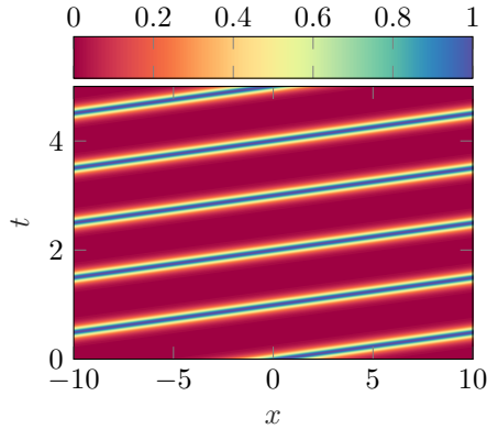
FIGURE 6.6. Evolution of the modulus of the soliton (6.12) for c = 20 and k = 0.81 .
