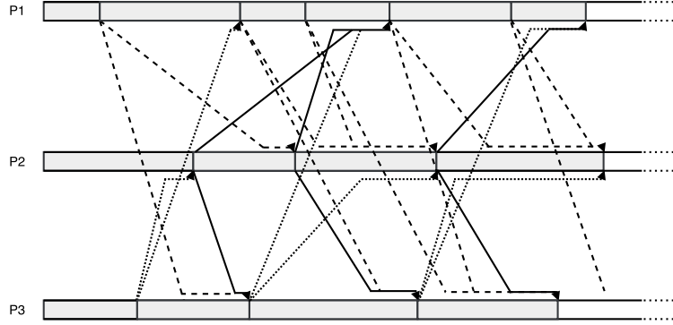
Figure 3: Example of the asynchronous two-stage iteration with flexible communication.
