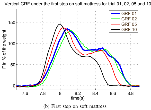
Fig. 4: Example of vertical Ground Reaction Forces (GRF) under the foot stepping (a) before and (b) after the transition from hard ground to soft mattress. The trials are time-aligned in order to align the first peak of the last step on hard ground.
