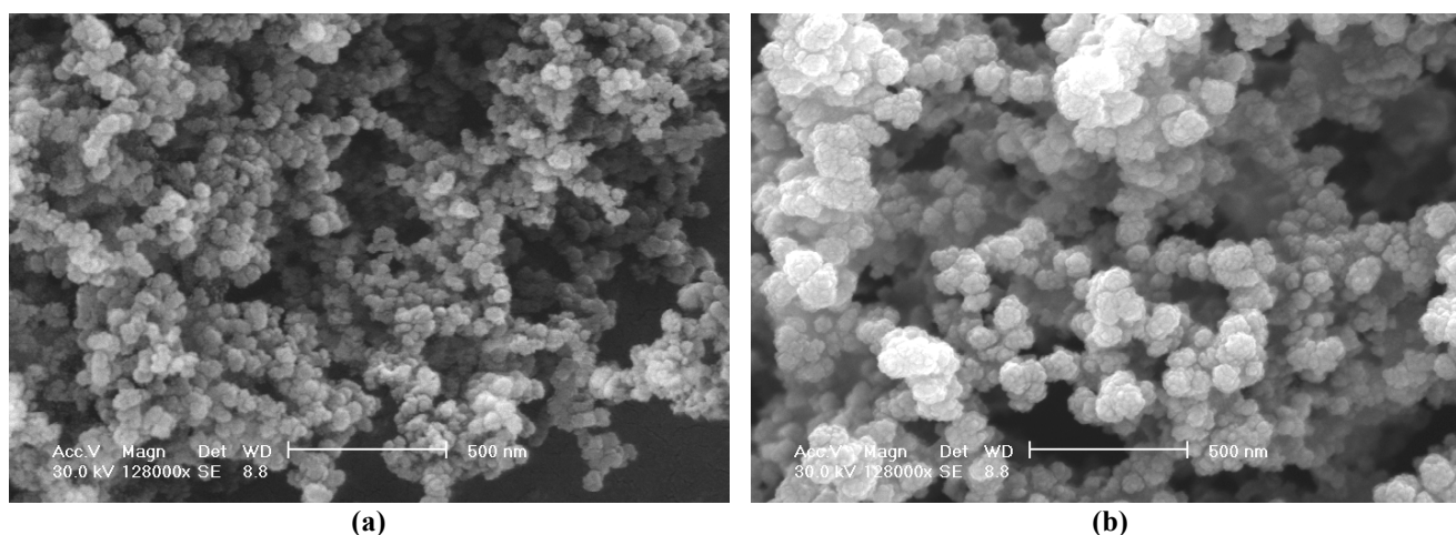
Figure 3 : ESEM images of Aerosil® 90 coated with ECN7 x 128 000 - Working conditions P = 8.5 MPa, T = 323 K - capillary size 100 \mu m - (a) uncoated Aerosil® 90 (b) coated nanoparticles
