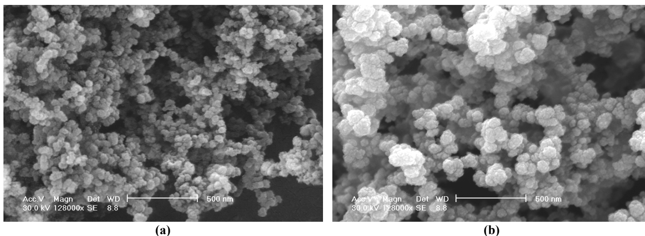
Figure 3 : ESEM images of Aerosil® 90 coated with ECN7 x 128 000 - Working conditions P = 8.5 MPa, T = 323 K - capillary size 100 µm - (a) uncoated Aerosil® 90 (b) coated nanoparticles
